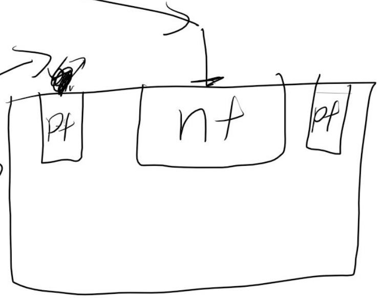
Cross-sectional view
