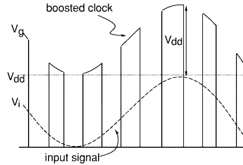
Fig. 8. Conceptual bootstrap circuit output.
