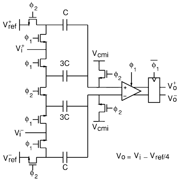
Fig. 10. Differential comparator.
